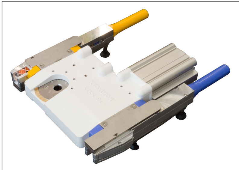
Tip changer with STC magazines installed
