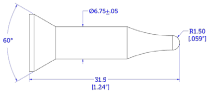
M06 Weld Pin
