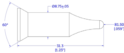
M08 Weld Pin
