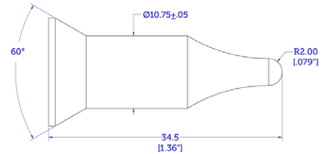
M10 Weld Pin
